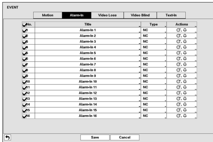
Figure 18: Event – Alarm-In setup screen.
