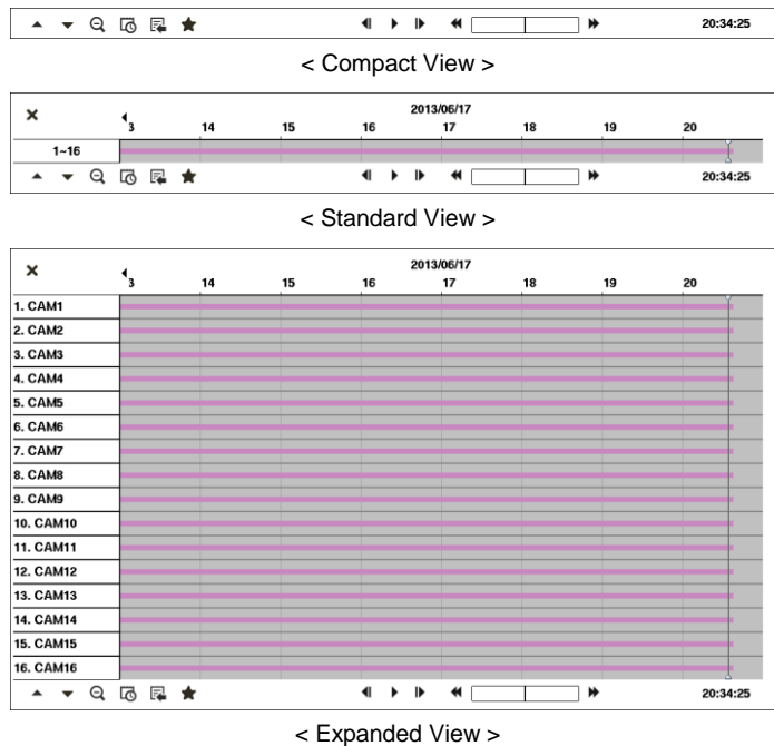
Figure 49: Record Table Search screen.
