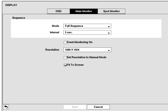
Figure 40: Display – Main Monitor setup screen.
