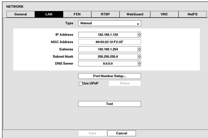
Figure 28: Network – LAN setup screen.
