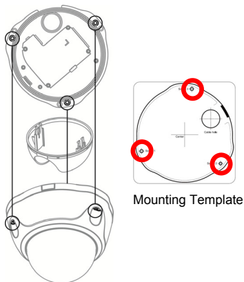
< Vandal Dome Model >
